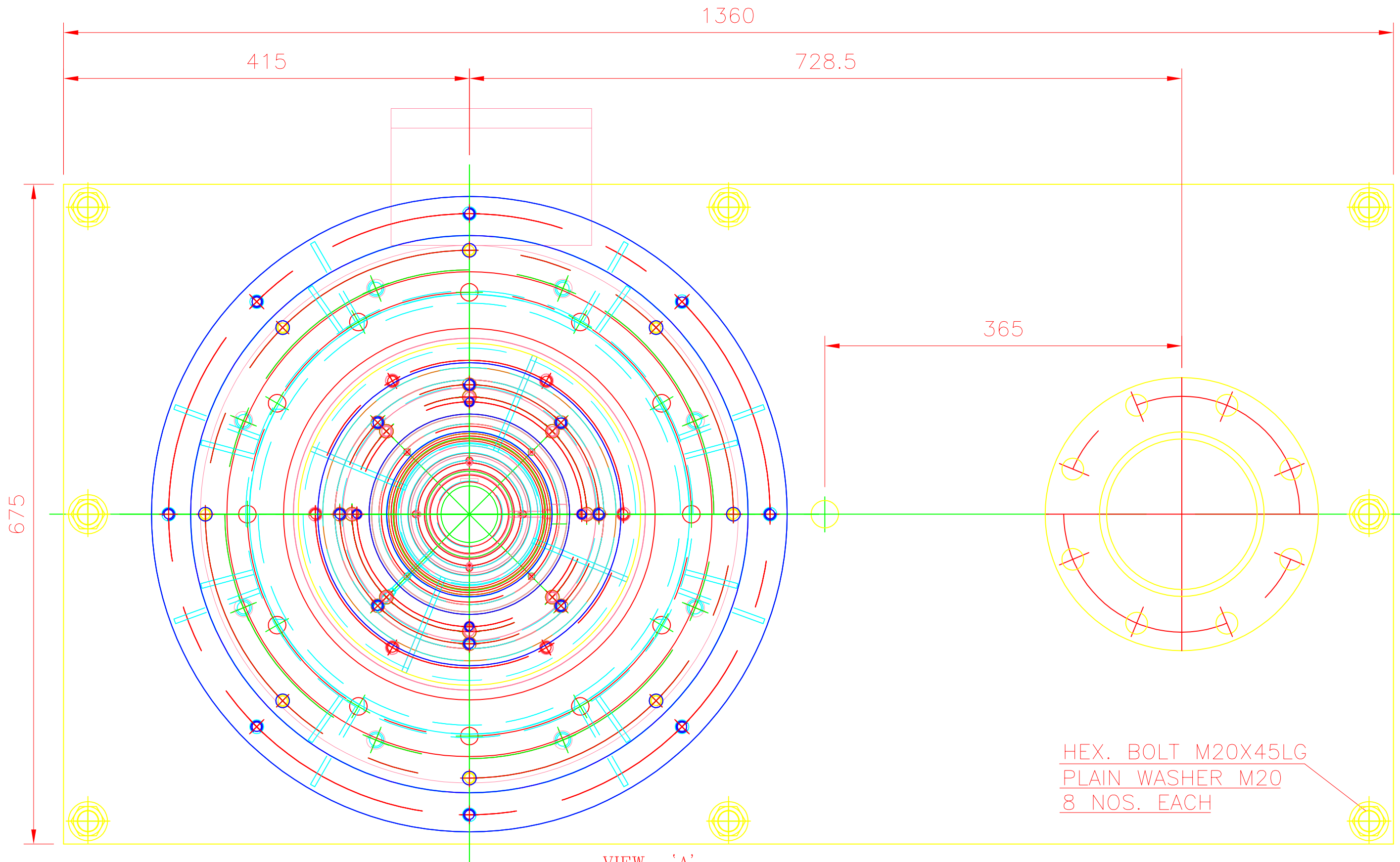
VIEW - 'A' (FROM SHT.NO.1)
