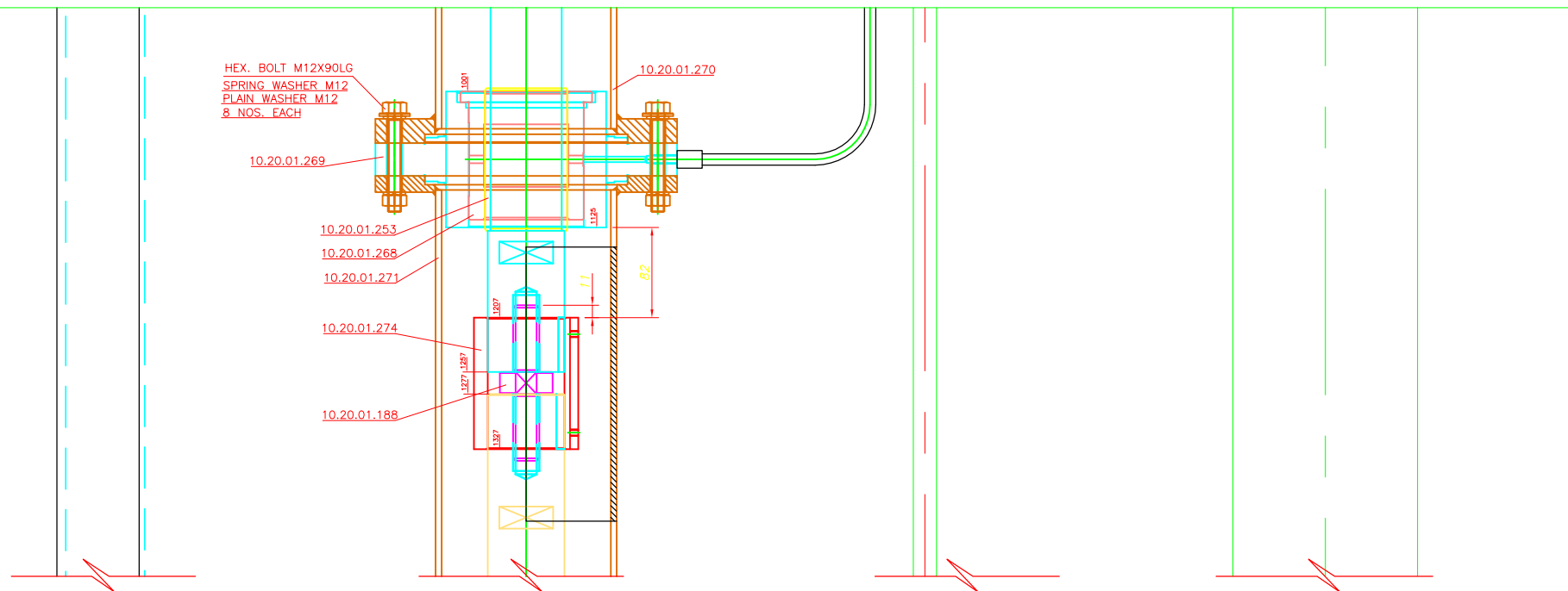
ENLARGED VIEW - 'Z' (FROM SHT.NO.1)
